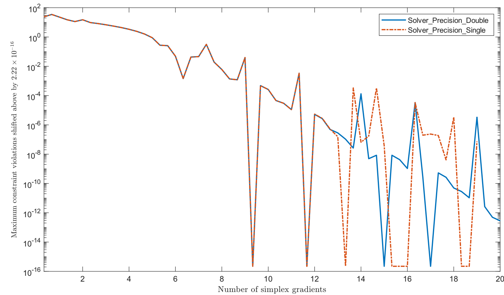
Solving "HS11" with "plain" feature
