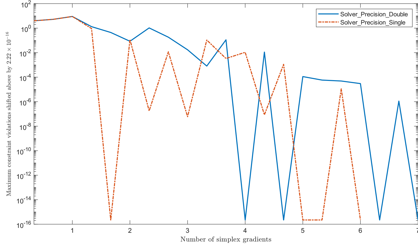
Solving "HS14" with "plain" feature
