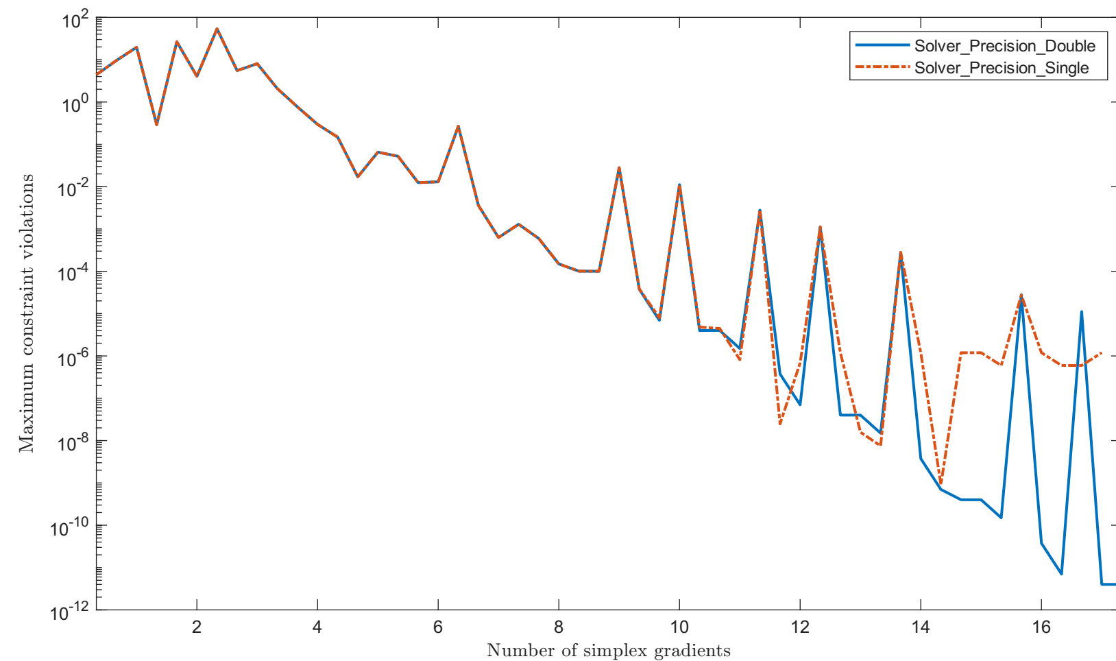
Solving "HS6" with "plain" feature
