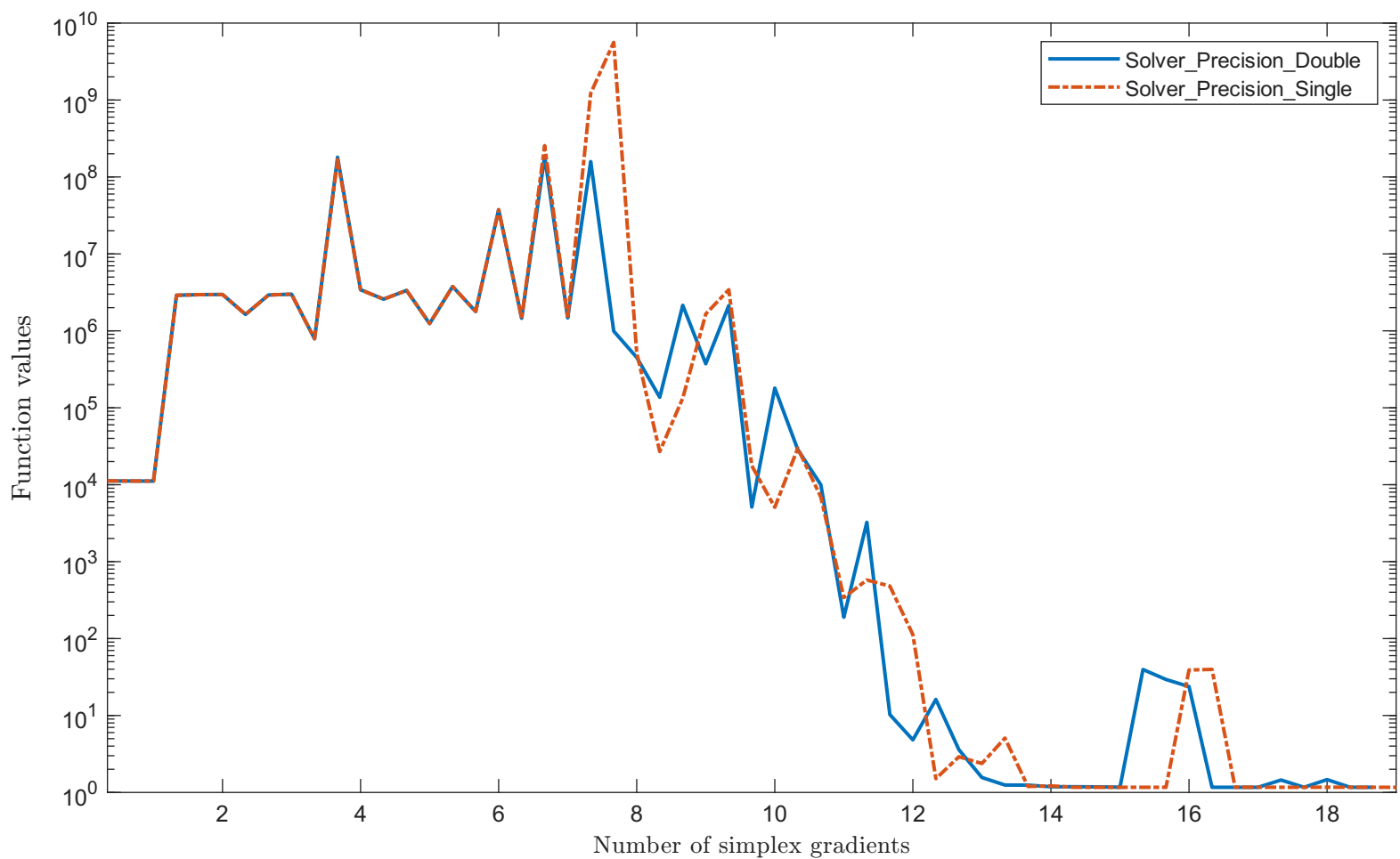
Solving "MISRA1DLS" with "plain" feature
