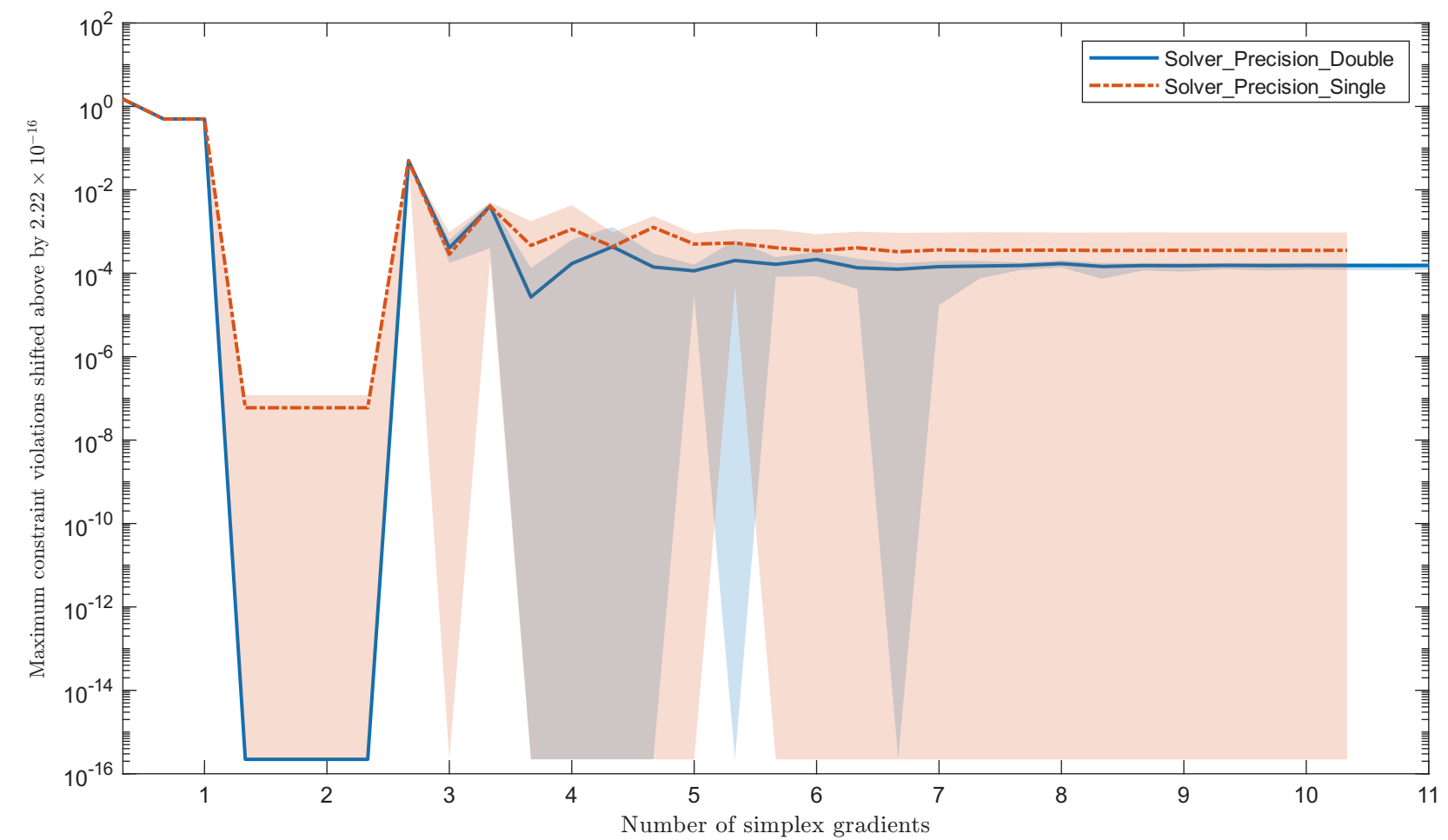
Solving “HS20” with “noisy_0.001_mixed_gaussian” feature
