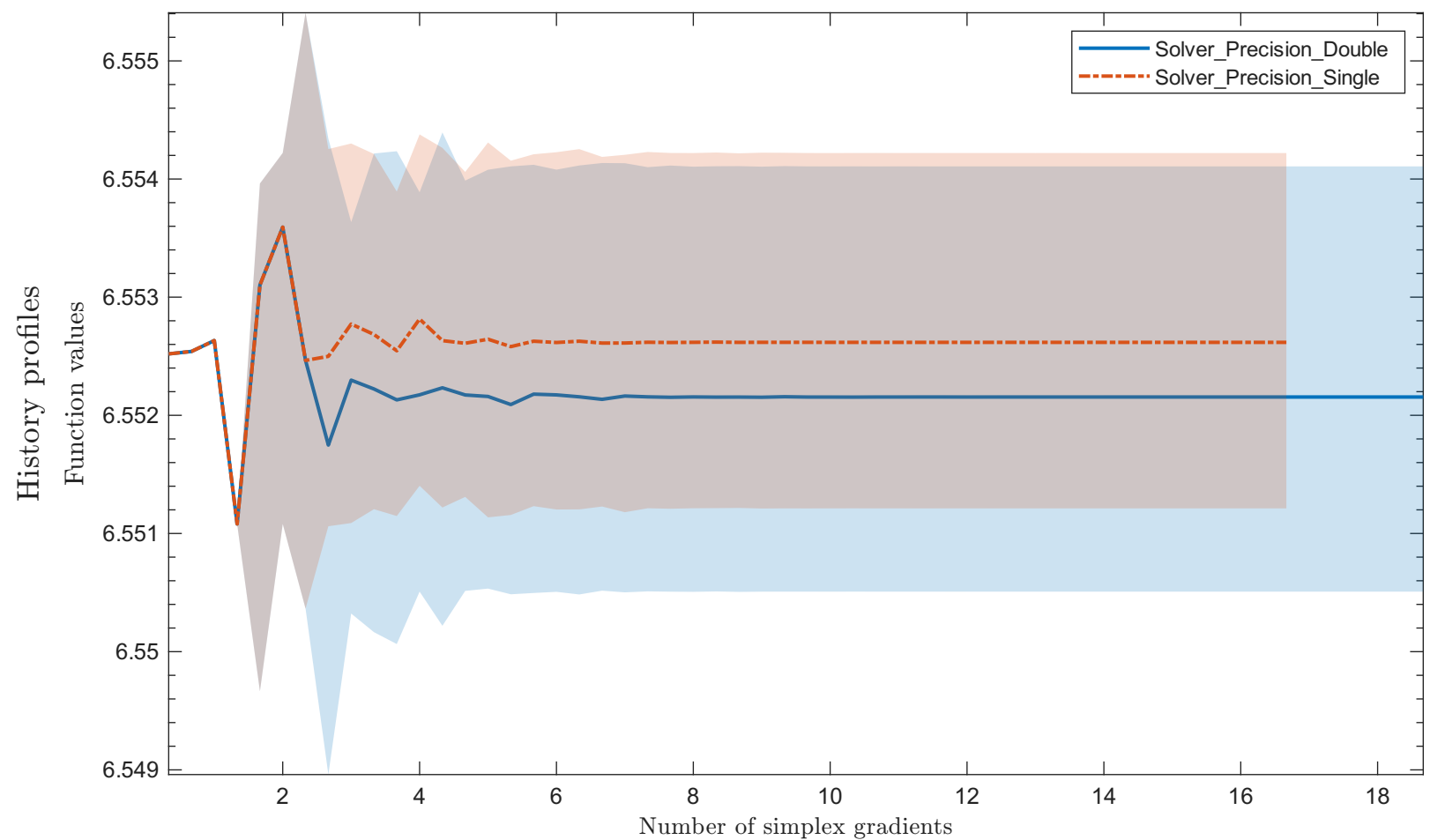
Solving “LOGHAIRY” with “noisy_0.001_mixed_gaussian” feature
