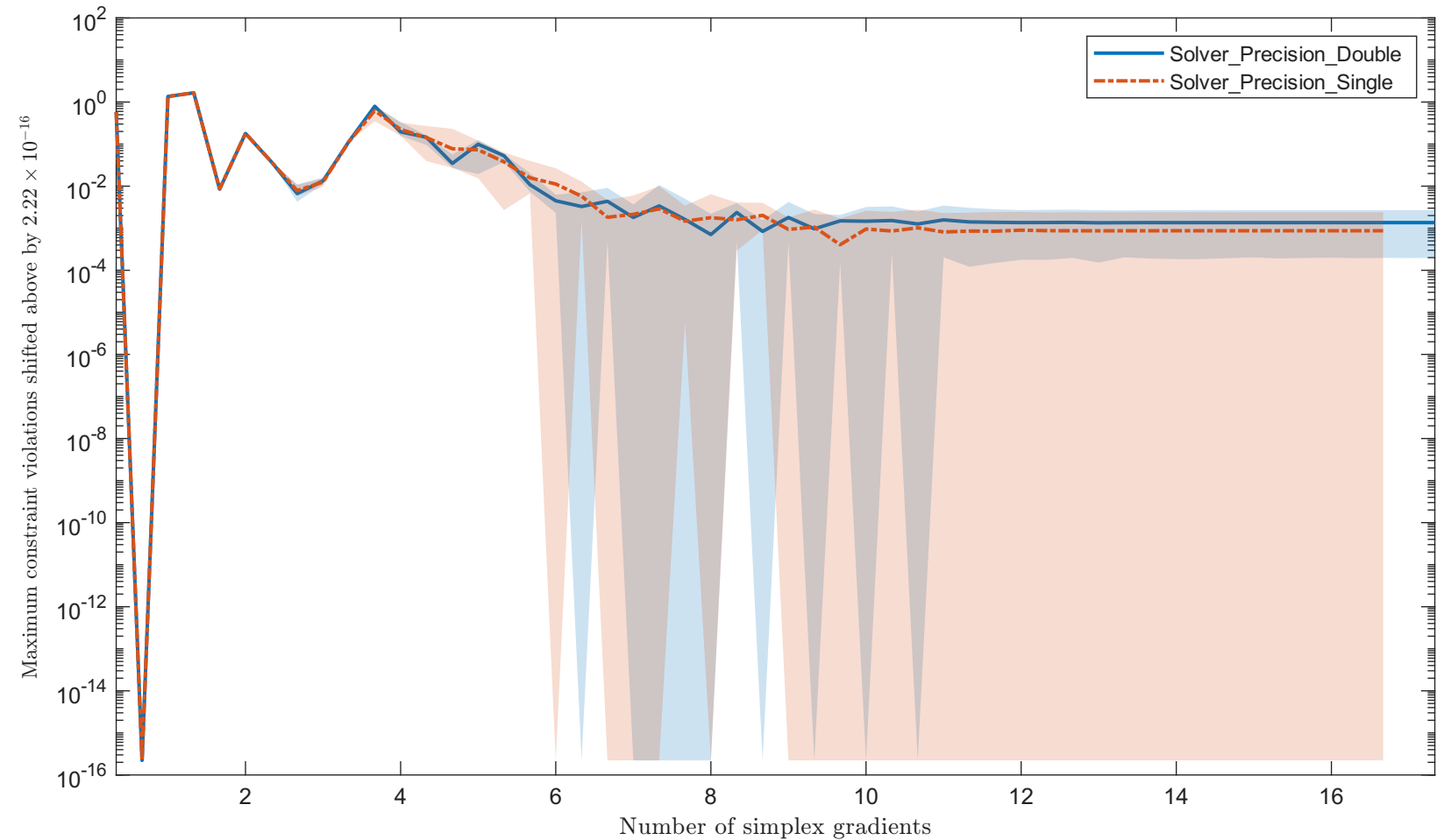
Solving "TWOBARS" with "noisy_0.001_mixed_gaussian" feature
