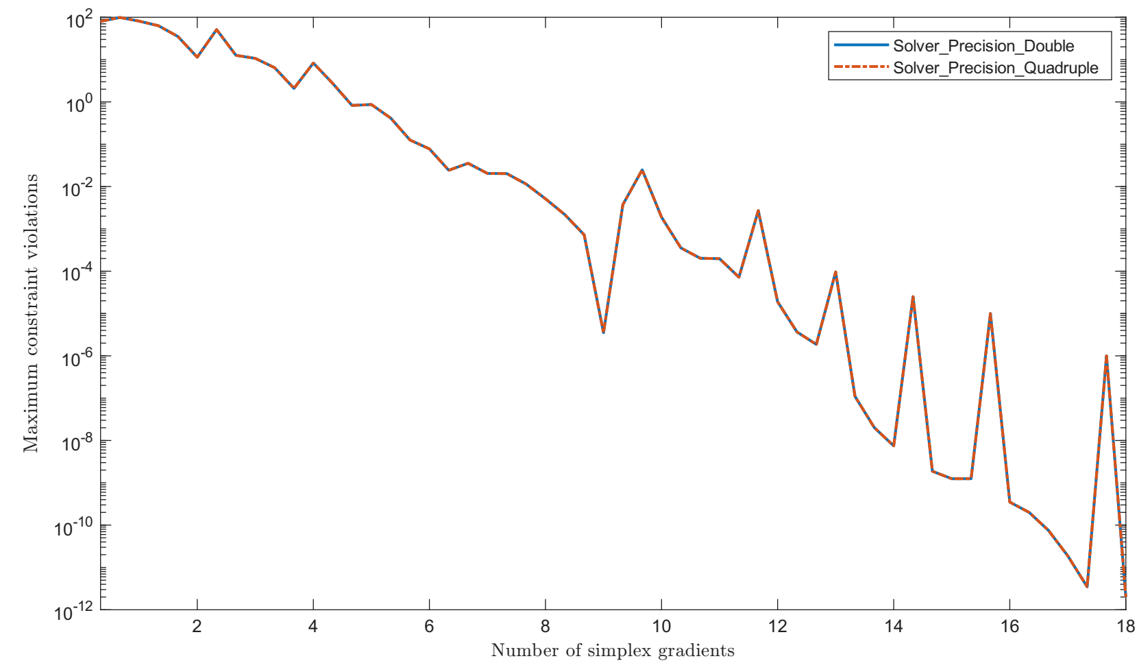
Solving "TRYmB" with "plain" feature
