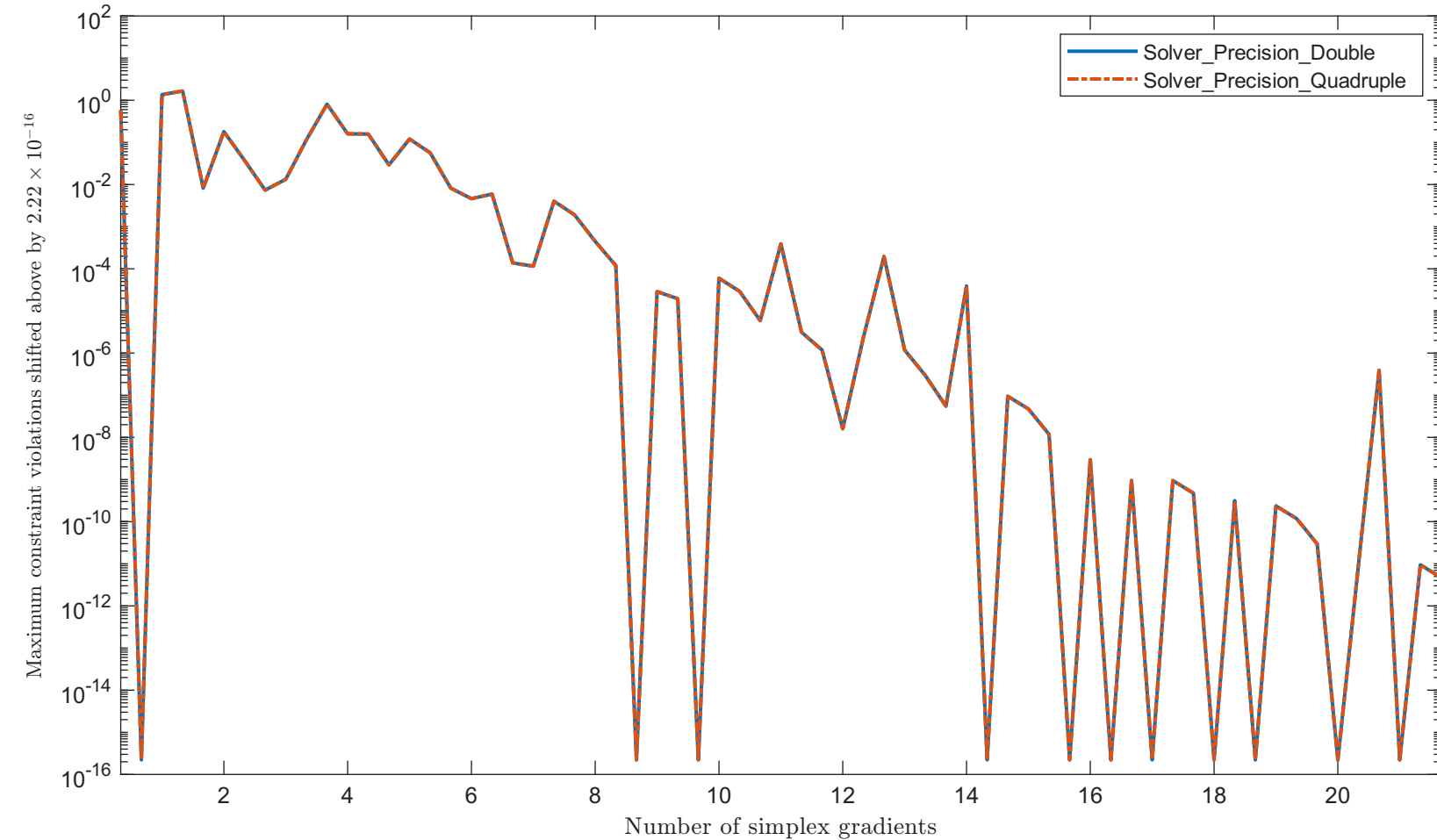
Solving “TWOBARS” with “plain” feature
