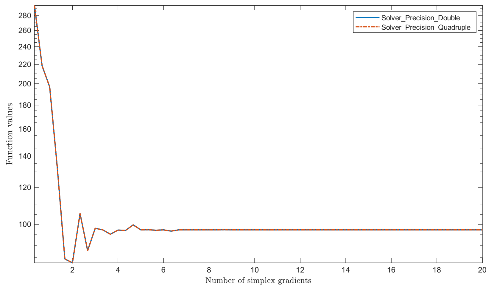
History profiles
