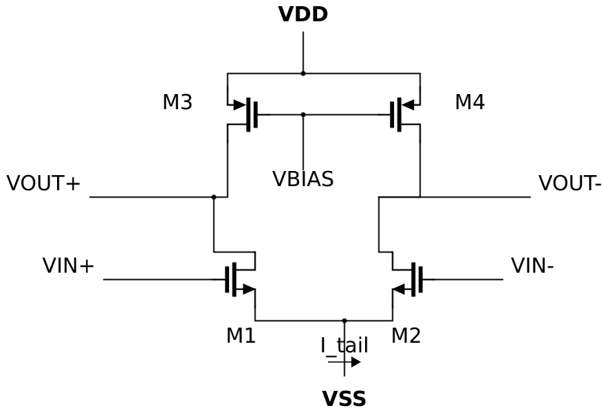
Original matched differential stage
