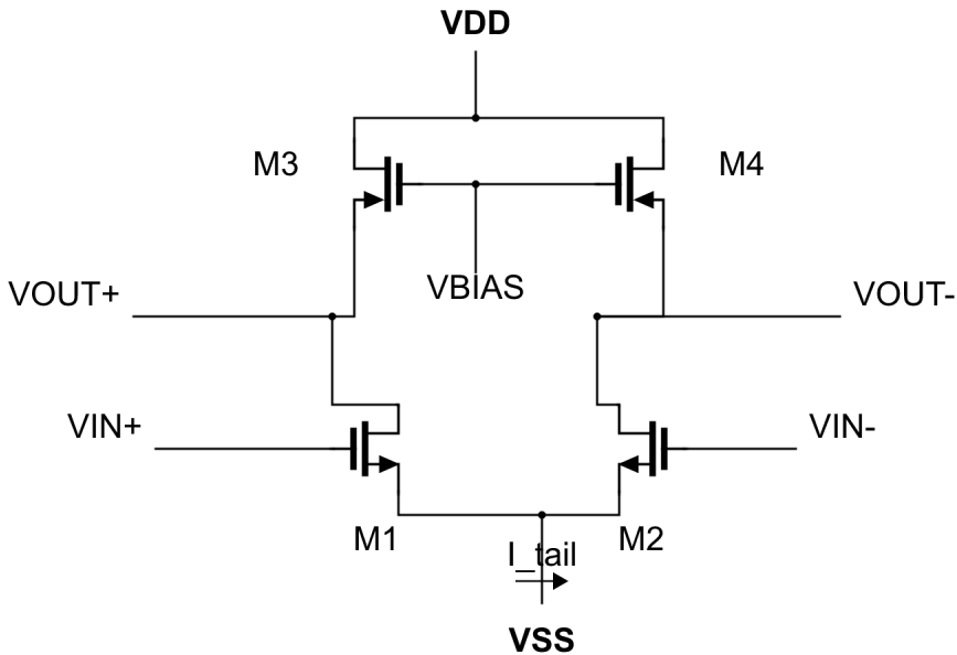
Original matched differential stage
