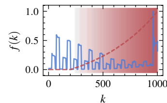
(o) OmniAnomaly
