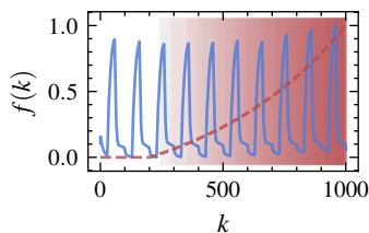
(l) IForest
