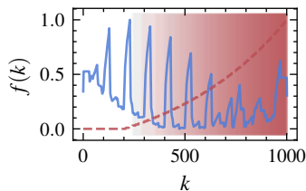
(p) TranAD
