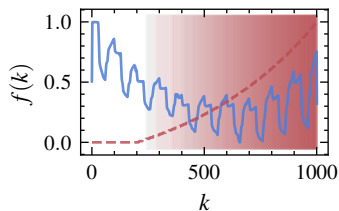
(r) DeepSVDD
