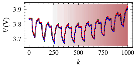
(e) LSTMAD
