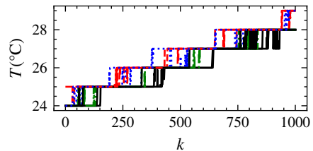
(g) UKF-WLGLR
