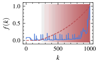
(i) EKF-WLGLR
