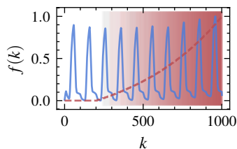
(m) GMM
