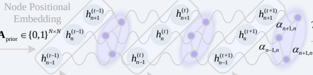
Node-wise Transformer
