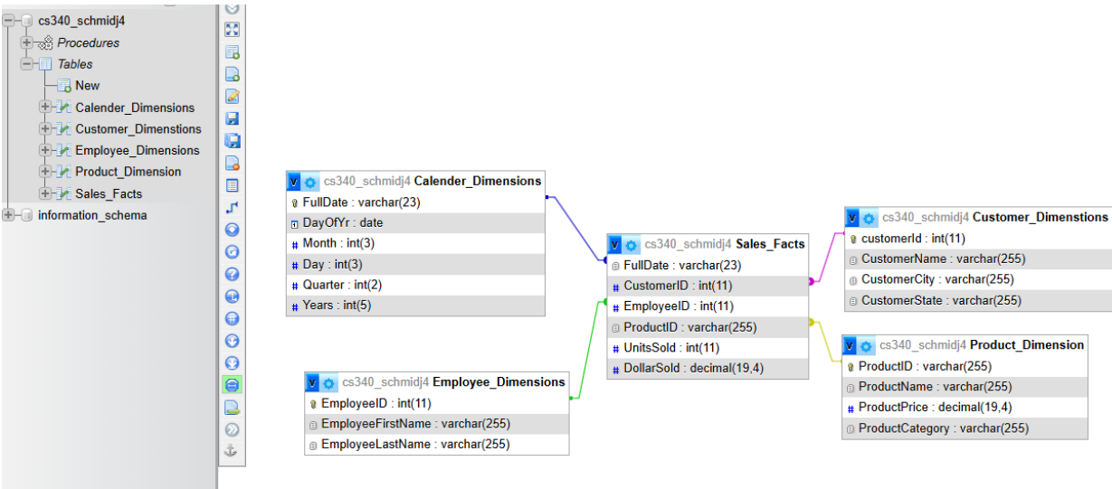
Analytical DB Schema
