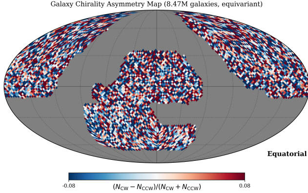
Figure 1. Equivariant chirality asymmetry map of the full 8.47 M-galaxy catalog (Mollweide projection, equatorial coordinates; per-pixel asymmetry A_p = (N_{CW} - N_{CCW}) / (N_{CW} + N_{CCW}) = 2(f_{CW,p} - \frac{1}{2}) at HEALPix NSIDE = 64, color scale [-0.08, +0.08] on the 24,087-pixel FSC support ( f_{sky} = 0.49005 ; Sec. 2.1). This is the full-catalog map, a broader footprint than the 23,633-pixel, 887,472-galaxy HC-RI support used for the primary dipole fit below; no coherent large-scale structure is visually apparent in either support.
