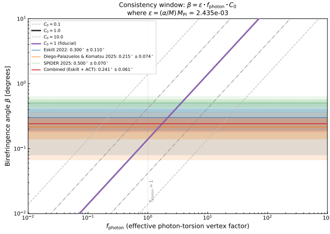
FIG. 3. Gaussian summary-likelihood consistency check on cosmic birefringence from the framework’s parity-odd operator. The photon-torsion vertex factor f_{\text{photon}} (for C_0 = 1 ) required for the coupling \alpha/M \approx 10^{-21} \text{ GeV}^{-1} to reproduce the observed birefringence angle. Horizontal bands show measurements from Planck NPIPE [30] and ACT DR6 [34]; the combined posterior gives \beta = 0.241^\circ \pm 0.061^\circ ( 3.9\sigma , BF \approx 176 ). The implied f_{\text{photon}} \times C_0 = 1.73 \pm 0.44 is \mathcal{O}(1) , indicating no fine-tuning is required. This is a summary-likelihood consistency check using published \beta values, not a map-level CMB analysis.
