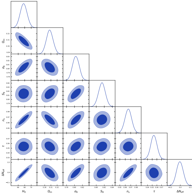
FIG. 3. Full-tension MCMC corner plot (119,617 post-burnin samples, a getdist -thinned slice of the 176,840 raw samples reported in Table II; see footnote 4) over the joint Planck+BAO+SN+H0+ S_8 combination. Marginal posteriors for H_0 , \Omega_m , \sigma_8 , S_8 , and \Delta N_{\text{eff}} are shown on the diagonal; 2D contours at 1\sigma and 2\sigma levels off-diagonal. The \Delta N_{\text{eff}} posterior is consistent with zero ( -0.020 \pm 0.169 ), confirming that the spin-torsion framework does not inject additional relativistic species at recombination.
