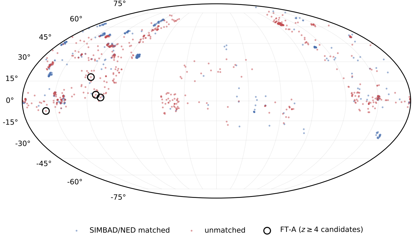
FIG. 4. Sky distribution of the released catalogue in equatorial coordinates, split by SIMBAD/NED counterpart status, with the four FT-A high-redshift candidates circled. The pattern traces DR1 tiling, not any property of the score.
