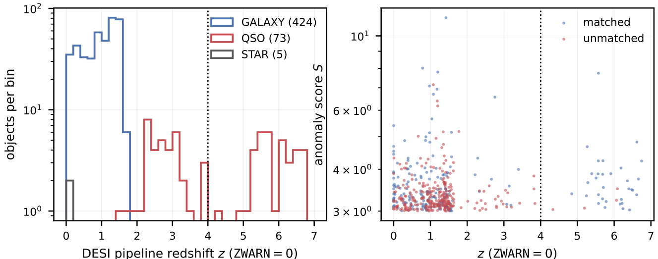
FIG. 3. Left : DESI pipeline redshifts of the 502 objects with ZWARN = 0 , by pipeline classification; the z = 4 line marks the FT-A tier boundary. Right : score against redshift for the same subset. High score and high redshift are not the same population.
