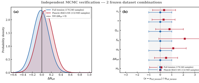
FIG. 2. \Delta N_{\text{eff}} marginal posterior comparison across the two frozen dataset combinations of Table II (176,240 and 132,949 samples). Panel (a): Gaussian summaries of the \Delta N_{\text{eff}} marginal posteriors at the Table II means \pm 1\sigma , with the Standard-Model value \Delta N_{\text{eff}} = 0 marked. Panel (b): all seven Table II parameters, normalized to the full-tension mean and \sigma . Both combinations recover \Delta N_{\text{eff}} consistent with zero at < 1\sigma ; the headline “full-tension” stack (Planck+BAO+SN+ H_0 + S_8 ) gives \Delta N_{\text{eff}} = -0.020 \pm 0.169 . No evidence for a recombination-era \Delta N_{\text{eff}} shift appears in this stock-CAMB proxy run; this does not directly test the ECH spin-torsion sector, which lacks a Boltzmann-module prediction for \Delta N_{\text{eff}} in stock-CAMB (see § III scope note).
