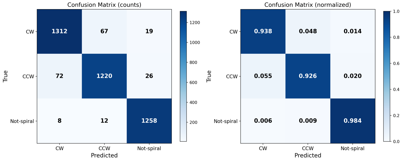
FIG. 6. Confusion matrix for the 3-class ViT-Small classifier on the validation set ( N = 3,994 ). Left : Raw counts. Right : Row-normalized fractions. The dominant error mode is CW \leftrightarrow CCW misclassification ( \sim 5\% swap rate), consistent with ambiguous spiral morphology in face-on galaxies. Not-spiral classification is highly reliable (96.5% precision), confirming that the three-class design successfully routes non-spirals to the rejection class.
