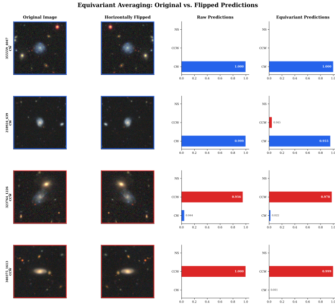
FIG. 5. Demonstration of the flip-equivariance consistency loss. For each galaxy image x , the model is trained to satisfy p_{\text{CW}}(x) \approx p_{\text{CW}}(\mathcal{F}[x]) . The raw model achieves flip-swap correlation r = 0.833 ; test-time equivariant averaging (averaging predictions on the original and flipped image) recovers r = 1.000 exactly.
