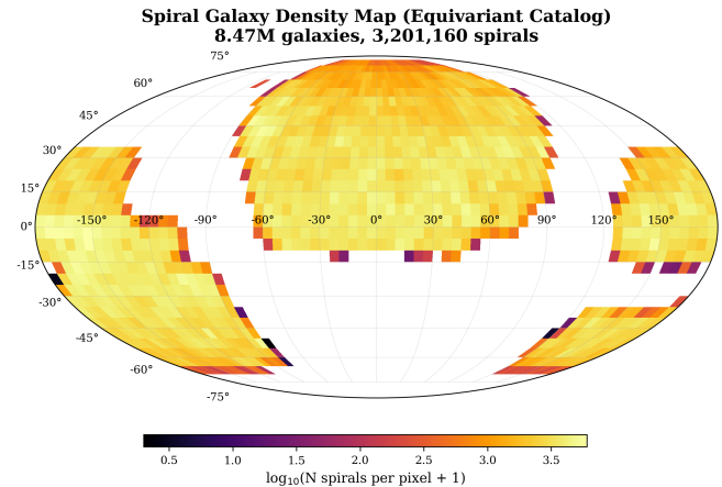
FIG. 1. Sky distribution of spiral galaxy density across the DESI Legacy Imaging Survey DR8 footprint in equatorial coordinates. The catalog spans \sim 14,000 \text{ deg}^2 , with density variations reflecting the combined DECaLS, BASS, and MzLS survey geometry.
