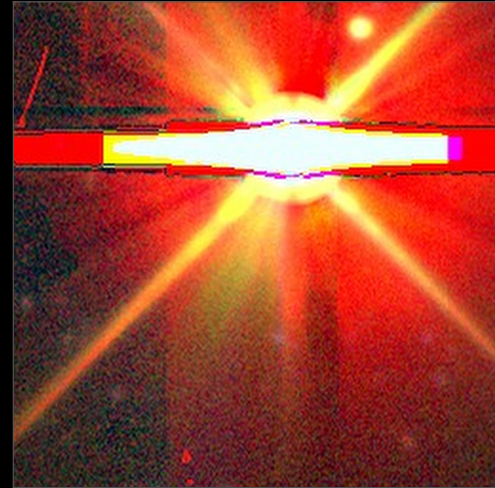
FIG. 4. NEOWISE top infrared anomaly at (\alpha, \delta) = (180.59^\circ, 0.56^\circ) , score = 11.5. DESI Legacy Survey DR9 grz composite, 256 \times 256 pixels ( 108'' \times 108'' ). Extreme W1–W2 infrared color excess; no prior SIMBAD entry within 5'' . The optical counterpart is a bright, saturated source with diffraction spikes indicative of a luminous red stellar or quasi-stellar object. Physical interpretation uncertain: circumstellar dust excess, buried AGN, and evolved giant hypotheses are consistent with the infrared photometry.
