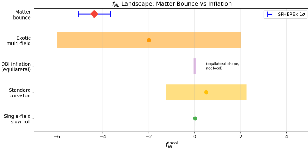
Figure 3: f_{NL} landscape: matter bounce vs. inflationary alternatives. The bounce prediction (red diamond) is parameter-free; inflationary alternatives require free parameters to reach the same region. SPHEREx 1\sigma error bar shown in blue.
