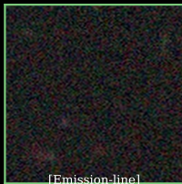
[Emission-line] RA 246.3°
