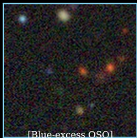
[Blue-excess QSO] RA 211.3°
