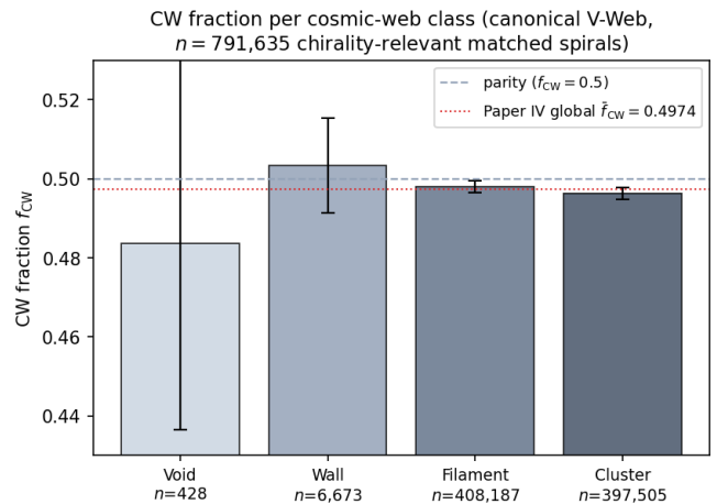
FIG. 3. CW fraction per cosmic-web class on the canonical V-Web run, on the n = 812,793 env-labeled spiral rows (791,635 unique chirality-relevant matched spirals; §VI A). Bars show the observed f_{\text{CW}} per class; black error bars are 95% Jeffreys binomial credible intervals. The void bin ( n = 428 ) is dominated by counting noise and brackets parity. The dashed horizontal line is parity ( f_{\text{CW}} = 0.5 ); the dotted red line is the Paper IV global \bar{f}_{\text{CW}} = 0.4974 classifier-monopole offset. All four classes bracket the Paper IV monopole, consistent with no environmental dependence beyond the catalog-wide classifier bias.
