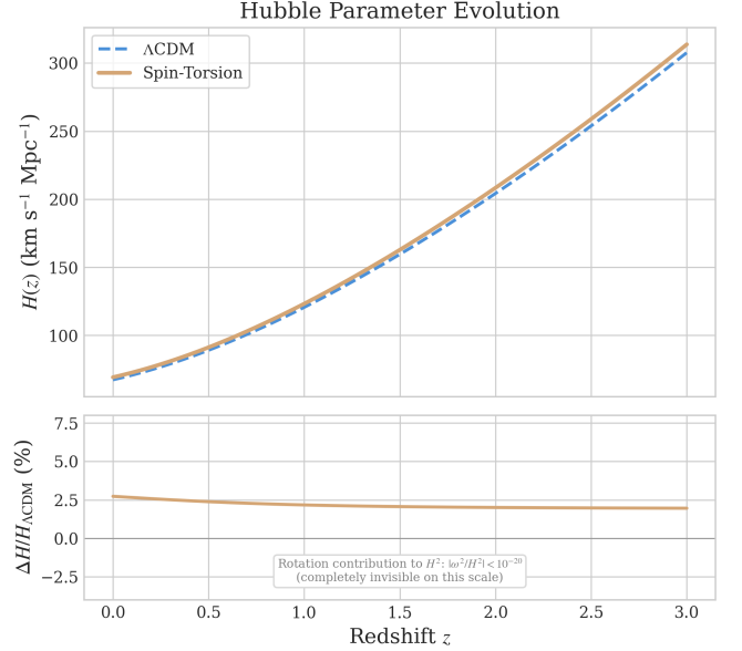
FIG. 3. Cosmic rotation \omega vs Hubble expansion H . Distance-impact of a residual cosmic rotation component on the late-time Hubble flow. The CMB isotropy bound (\omega/H)_0 < 5 \times 10^{-11} from Saadeh et al. [21] pins the rotation contribution to \Lambda_{\text{eff}} = c_\omega \omega^2 (Eq. 10) at the \lesssim 10^{-22} \rho_\Lambda^{\text{obs}} level — negligible at all redshifts. (The panel’s burned-in annotation quotes the equivalent bound as a fractional contribution to the expansion rate, |\omega^2/H^2| < 10^{-20} ; the two statements bound the same rotation term in different units.) The dark-energy mechanism in this paper is therefore the \Xi M_{\text{Pl}}^2 term sourced by the parity-odd contorsion sector (§II A 2), not the rotation component.
