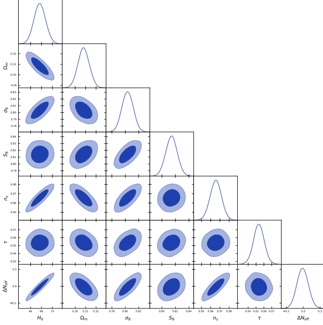
FIG. 4. Full-tension MCMC corner plot (119,617 post-burnin samples, a getdist -thinned slice of the 176,840 raw samples reported in Table II; see footnote 4) over the joint Planck+BAO+SN+H0+ S_8 combination. Marginal posteriors for H_0 , \Omega_m , \sigma_8 , S_8 , and \Delta N_{\text{eff}} are shown on the diagonal; 2D contours at 1\sigma and 2\sigma levels off-diagonal. The \Delta N_{\text{eff}} posterior is consistent with zero ( -0.020 \pm 0.169 ), confirming that the spin-torsion framework does not inject additional relativistic species at recombination.
