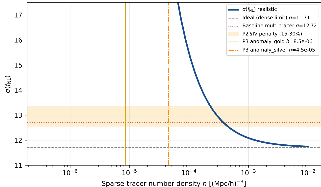
Multi-tracer Fisher: shot-noise sensitivity for sparse anomaly tracers
