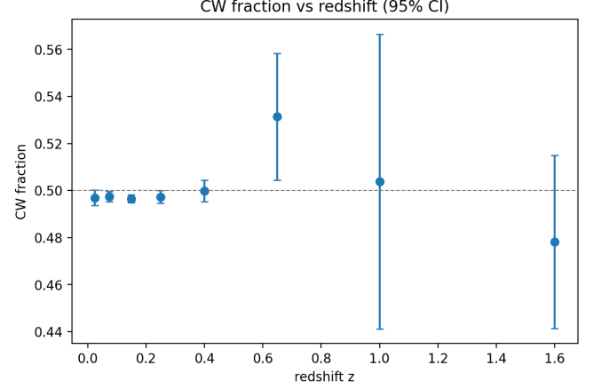
FIG. 4. Equivariant CW fraction versus redshift across the matched DR1 chirality-relevant sample, with 95% binomial confidence intervals per bin. The low- z bins that dominate the sample (median z = 0.168 ) sit on the 0.5 line; bins above z \approx 0.5 contain few objects and have correspondingly wide intervals. The binned values are consistent with no redshift dependence, in agreement with the label-shuffle permutation test ( p = 0.372 ) and the logistic regression in the text.
