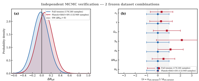
FIG. 2. \Delta N_{\text{eff}} marginal posterior comparison across the two frozen dataset combinations of Table I (176,240 and 132,949 samples). Panel (a): Gaussian summaries of the \Delta N_{\text{eff}} marginal posteriors at the Table I means \pm 1\sigma , with the Standard-Model value \Delta N_{\text{eff}} = 0 marked. Panel (b): all seven Table I parameters, normalized to the full-tension mean and \sigma . Both combinations recover \Delta N_{\text{eff}} consistent with zero at < 1\sigma ; the headline “full-tension” stack (Planck+BAO+SN+H0+ S_8 ) gives \Delta N_{\text{eff}} = -0.020 \pm 0.169 . No evidence for a recombination-era \Delta N_{\text{eff}} shift appears in this stock-CAMB proxy run; this does not directly test the ECH spin-torsion sector, which lacks a Boltzmann-module prediction for \Delta N_{\text{eff}} in stock-CAMB (see § III scope note).
