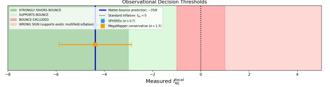
FIG. 6. Observational decision thresholds on the measured local-template f_{\text{NL}} (horizontal axis). Shaded regions, left to right: dark green — measurement near the -35/8 prediction, strongly favors the bounce; light green — negative f_{\text{NL}} of bounce-compatible magnitude, supports the bounce; dark red (legend label “bounce excluded”) — measurement consistent with zero, disfavoring the quasi-dust matter bounce while remaining consistent with standard single-field inflation; light red — positive f_{\text{NL}} , disfavoring the bounce and instead supporting exotic multifield inflation. Blue vertical line: bounce prediction f_{\text{NL}} = -35/8 ; black dotted line: standard inflation f_{\text{NL}} \approx 0 . Error bars: SPHEREx ( \sigma = 0.7 ) and MegaMapper conservative ( \sigma = 1.5 , illustrative: between the \sigma \approx 0.5 ideal and the b_\phi -50% degraded \sigma \approx 2.2 of Sec. VII, not an independently calibrated forecast), both centered on the bounce prediction.
