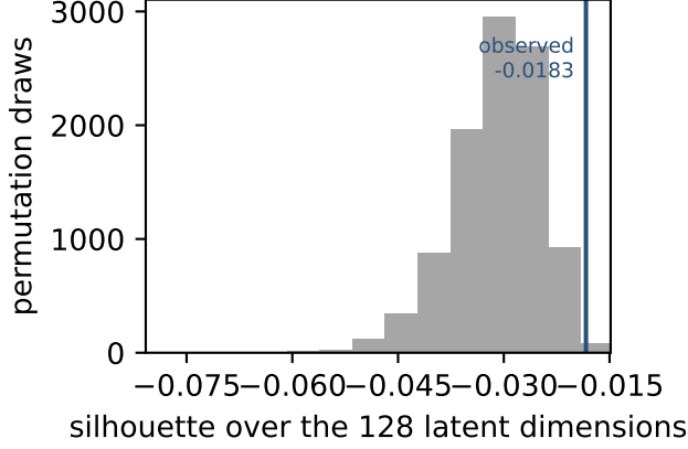
FIG. 8. Silhouette of the nine-family partition over the 128 latent dimensions, against its 10,000-draw label-permutation null. The observed value beats every draw but is itself negative: structured, but not separated.
