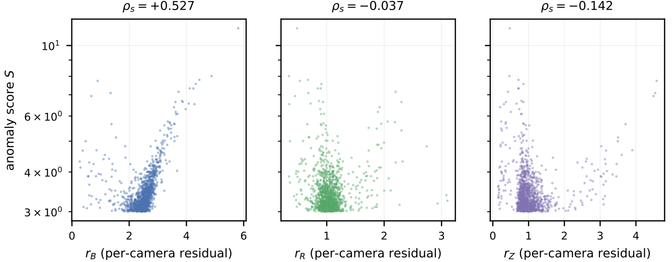
FIG. 6. Anomaly score against the per-camera reconstruction residual for the 1,244 released objects. The score tracks the b -camera residual; its dependence on r_R is consistent with zero ( \rho_s = -0.037 , p = 0.19 ) and its dependence on r_Z is small but significant ( \rho_s = -0.142 , p \approx 5 \times 10^{-7} ).
