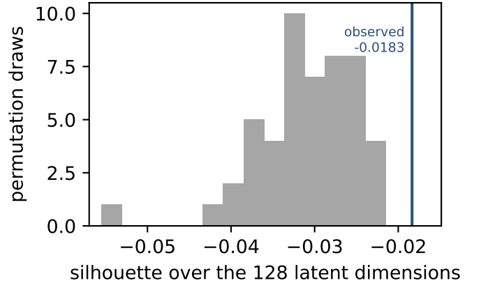
FIG. 8. Silhouette of the nine-family partition over the 128 latent dimensions, against its 50-draw label-permutation null. The observed value beats every draw but is itself negative: structured, but not separated.
