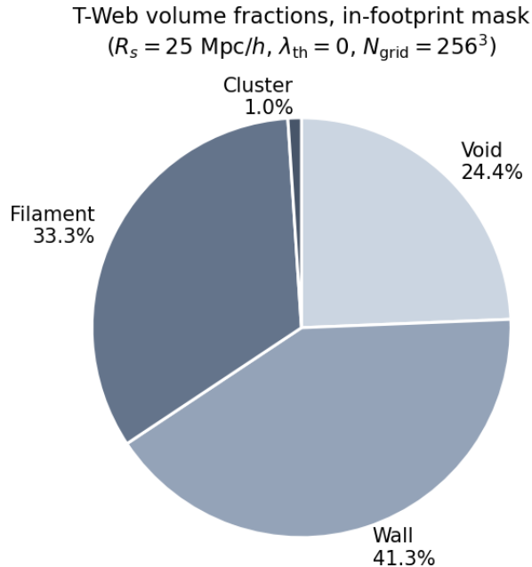
FIG. 2. In-footprint T-Web volume fractions for the canonical ( R_s = 25 \text{ Mpc}/h , \lambda_{\text{th}} = 0 , N_{\text{grid}} = 256^3 ) run on 14,622,283 DESI DR1 spectroscopic galaxies. The cluster volume fraction (1.0%) reflects the high-density tail; the wall+filament fraction (74.5%) dominates as expected for galaxy-traced large-scale structure.
