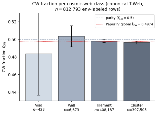
FIG. 3. CW fraction per cosmic-web class on the headline T-Web run, on the n = 812,793 env-labeled spiral rows (covering 783,820 of the 791,635 unique chirality-relevant matched spirals; 7,815 lack an environment row, §VI A). Bars show the raw observed f_{CW} per class (counts shown; monopole subtraction enters the \sigma_{vs\ monopole} column only); black error bars are 95% Jeffreys binomial credible intervals, drawn on the row-level parent — the 3.56% duplicate rows (28,973 of 812,793 env-labeled rows) violate strict i.i.d., but the worst-case design-effect inflation of the interval widths is \sqrt{812,793/783,820} = 1.018 , i.e. \leq 1.9\% , and the homogeneity \chi^2 is recomputed on the unique-spiral subset in §VI A. The void bin ( n = 428 ) is dominated by counting noise and brackets parity. The dashed horizontal line is parity ( f_{CW} = 0.5 ); the dotted red line is the Paper IV global \bar{f}_{CW} = 0.4974 classifier-monopole offset. All four classes bracket the Paper IV monopole, consistent with no environmental dependence beyond the catalog-wide classifier bias.
