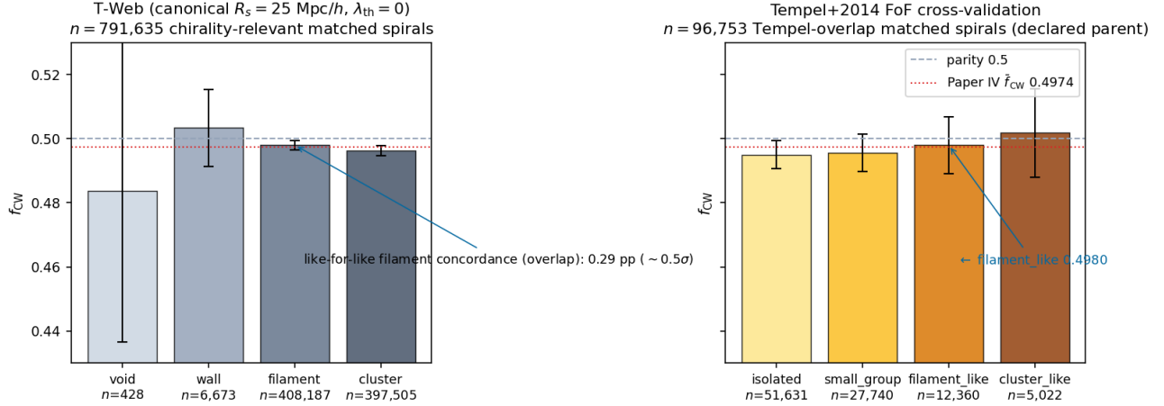
FIG. 9. T-Web (left; full-sample canonical run, shown as reference) vs Tempel+2014 FoF (right; 96,753-spiral overlap) cross-validation: per-class CW fraction with 95% Jeffreys binomial credible intervals, shared y-axis [0.43, 0.53]. Dashed reference is parity f_{CW} = 0.5 ; dotted-red reference is the Paper IV global \bar{f}_{CW} = 0.4974 classifier-monopole offset. The quantitative concordance statistic is computed like-for-like on the common overlap sample (§IX B): Tempel filament_like f_{CW} = 0.4980 ( n = 12,360 ) vs T-Web filament-on-overlap f_{CW} = 0.5009 ( n = 16,701 ), a 0.29 pp ( \sim 0.5\sigma ) difference, statistically indistinguishable (supporting, not load-bearing; the primary cross-classifier validation is the on-DESI DESIVAST re-projection in §VIII). Lower- n classes scatter by counting statistics and classifier-definition mismatch (T-Web \lambda_{th} = 0 vs Tempel discrete richness thresholds) but do not contradict the environmental-independence headline.
