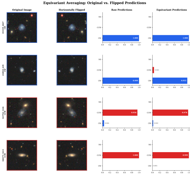
FIG. 5. Demonstration of the flip-equivariance consistency loss. For each galaxy image x , the model is trained to satisfy p_{CW}(x) \approx p_{CW}(\mathcal{F}[x]) . The raw model achieves flip-swap correlation r = 0.833 ; test-time equivariant averaging (averaging predictions on the original and flipped image) recovers r = 1.000 exactly.
