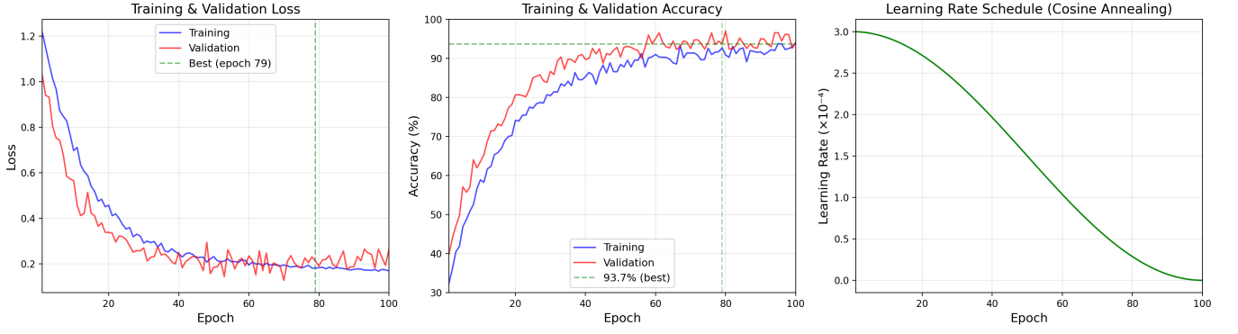
FIG. 4. Training and validation curves for the ViT-Small chirality classifier. Left : Cross-entropy loss converges within \sim 40 epochs, with validation loss minimum at epoch 79. Mild overfitting is visible after epoch 80. Center : Classification accuracy reaches 93.7% on the validation set at epoch 79. Right : Cosine annealing learning rate schedule from 3 \times 10^{-4} to \sim 10^{-7} .
