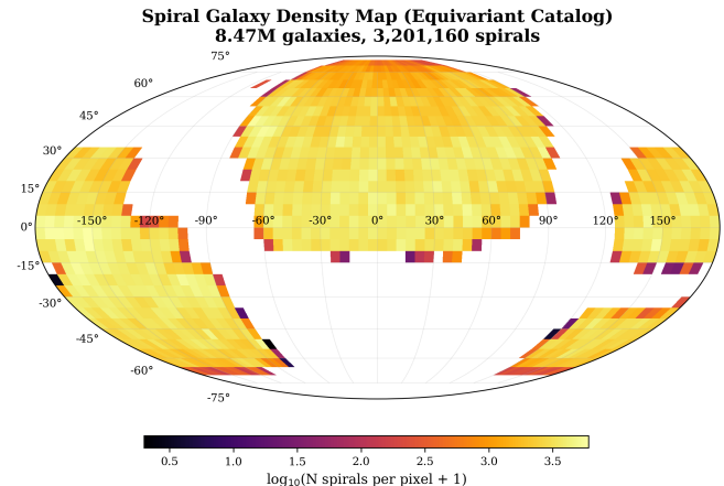
FIG. 1. Sky distribution of spiral galaxy density across the DESI Legacy Imaging Survey DR8 footprint in equatorial coordinates. The catalog spans \sim 14,000 deg 2 , with density variations reflecting the combined DECaLS, BASS, and MzLS survey geometry.
