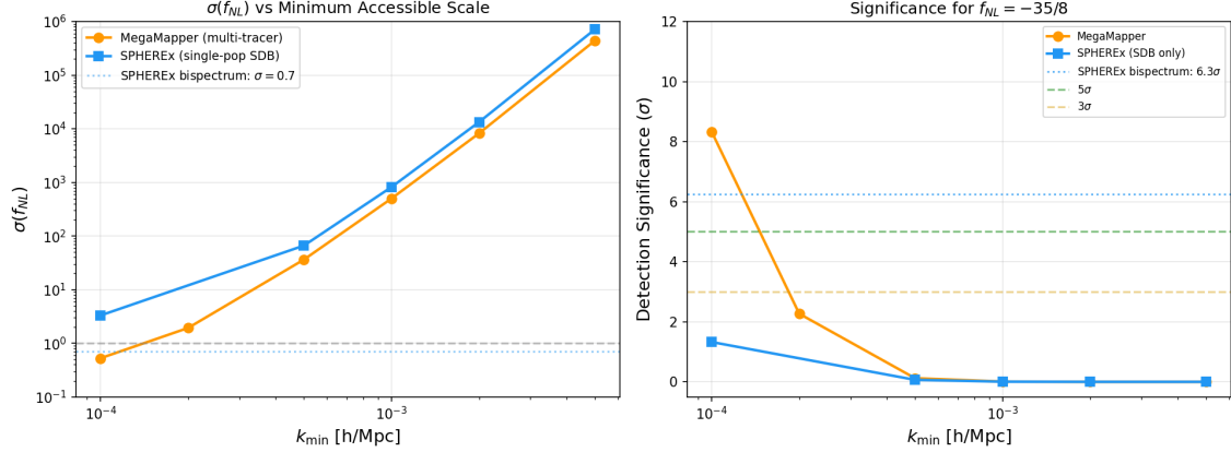
Figure 4: Left: \sigma(f_{NL}) vs. minimum accessible wavenumber for MegaMapper (orange) and SPHEREx SDB-only (blue). The SPHEREx bispectrum channel ( \sigma = 0.7 , dotted) avoids the ultra-large-scale fragility. Right: corresponding detection significance for f_{NL} = -35/8 .
