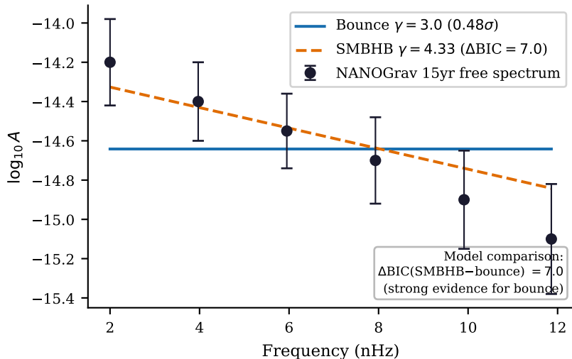
NANOGrav 15yr GWB free-spectrum fit
