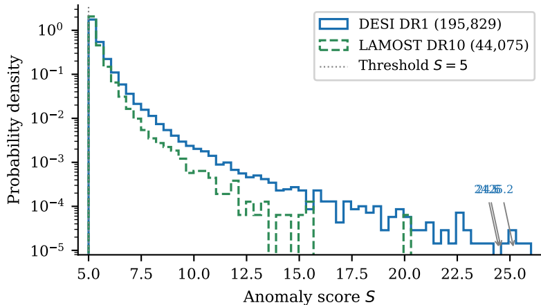
DESI DR1 and LAMOST DR10
