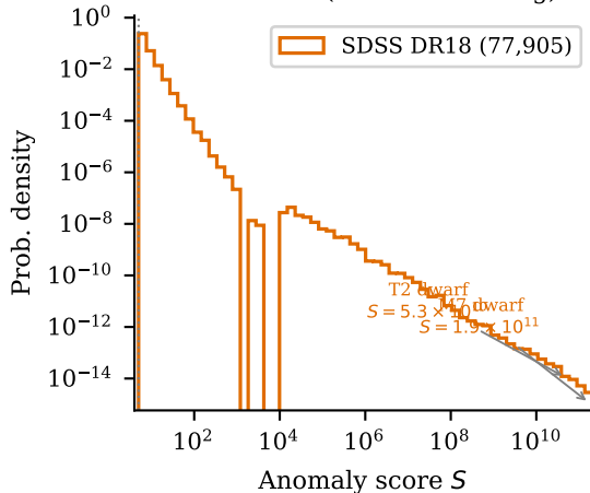
SDSS DR18 (transfer learning)
