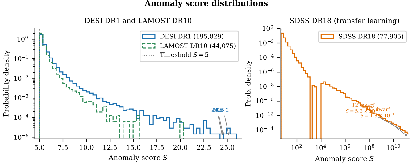
FIG. 3. Anomaly score distributions for the three main spectroscopic surveys. The score S is the per-spectrum reconstruction MSE rescaled to validation z -units: S = (\text{MSE} - \mu_{\text{val}}) / \sigma_{\text{val}} , where \mu_{\text{val}} and \sigma_{\text{val}} are the mean and standard deviation of MSE on the held-out 20% validation split of the per-survey training pool (§II B; cross-transfer for SDSS, native for DESI/LAMOST). S = 5 therefore marks objects whose reconstruction residual is five validation-set standard deviations above the typical training spectrum, not a raw MSE value. Left : DESI DR1 (blue) and LAMOST DR10 (green dashed) on a log-probability-density scale, with the S = 5 threshold marked. Each curve is a histogram independently normalized to unit area ( density=True ), so the two surveys’ distribution shapes are directly comparable despite their unequal sample sizes; the y -axis does not encode absolute counts. Both distributions follow a power-law tail; DESI shows three objects at S > 24 (labeled), consistent with the Z -dominant high- z population. Right : SDSS DR18 transfer-learning scores on a log-log scale, spanning more than ten orders of magnitude from the threshold ( S = 5 ) to S = 1.9 \times 10^{11} for the extreme-score M7 and T2 dwarfs. The extreme dynamic range of SDSS is a cross-transfer artifact (DESI-trained BiGAE applied to SDSS spectra outside the DESI training distribution); the SDSS native re-score (§III C) compresses the same objects to S < 14 , eliminating the 10^4 – 10^{11} tail. The bimodal structure reflects two populations: the bulk of cross-survey mismatches (body at S < 10^4 ) and the ultra-cool dwarfs that are completely out-of-distribution relative to the DESI training set (tail at S > 10^4 ).
