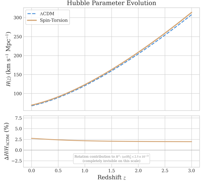
FIG. 3. ECH dark-energy model vs. \Lambda CDM Hubble evolution. Upper panel: Hubble parameter H(z) for the full ECH dark-energy model (orange; \Xi M_{\text{Pl}}^2 term from Eq. 10) versus \Lambda CDM (blue). Lower panel: percent deviation \Delta H/H_{\Lambda\text{CDM}} , reflecting the \Xi M_{\text{Pl}}^2 dark-energy mechanism—the central observable of this paper. The rotation contribution c_\omega \omega^2 is a distinct and negligible term: the CMB isotropy bound (\omega/H)_0 < 5 \times 10^{-11} from Saadeh et al. [21] confines it to \lesssim 10^{-21} \rho_\Lambda^{\text{obs}} ( (\omega/H)_0^2 < 2.5 \times 10^{-21} ; dividing by 3\Omega_\Lambda \approx 2.1 gives \sim 1.2 \times 10^{-21} of \rho_\Lambda^{\text{obs}} )—completely invisible on the scale plotted. The dark-energy mechanism in this paper is therefore the \Xi M_{\text{Pl}}^2 term sourced by the parity-odd contorsion sector (§II A 2), not the rotation component.
