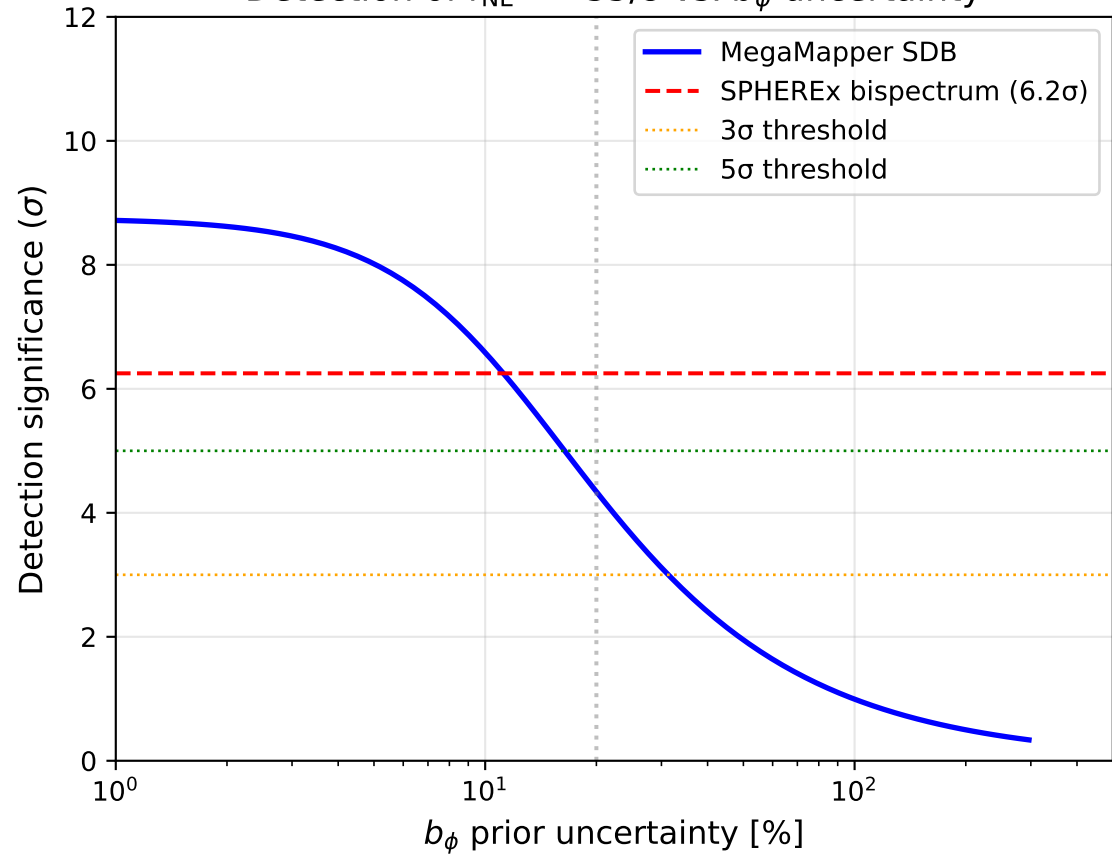
Detection of f_{\text{NL}} = -35/8 vs. b_\phi uncertainty
