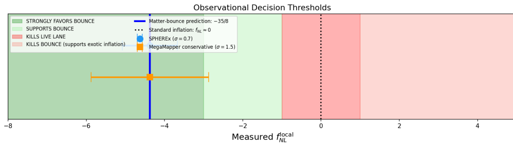
Figure 6: Observational decision thresholds. Green: strongly favors bounce. Red: kills the matter-bounce hypothesis. Blue vertical line: bounce prediction f_{\text{NL}} = -35/8 . Error bars: SPHEREx ( \sigma = 0.7 ) and MegaMapper conservative ( \sigma = 1.5 ).
