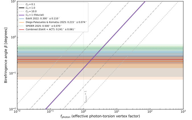
FIG. 3. Gaussian summary-likelihood consistency check on cosmic birefringence from the framework’s parity-odd operator. The photon-torsion vertex factor f_{\text{photon}} (for C_0 = 1 ) required for the coupling \alpha/M \approx 10^{-21} \text{ GeV}^{-1} to reproduce the observed birefringence angle. Horizontal bands show measurements from Planck NPIPE [31] and ACT DR6 [35]; the simplified inverse-variance combination gives \beta = 0.241^\circ \pm 0.061^\circ (3.9 \sigma auxiliary cross-check only; \text{BF} \approx 176 ). The headline observational constraint adopted in this paper is the published Eskilt et al. joint Planck+ACT analysis \beta = 0.342^\circ \pm 0.094^\circ (3.6 \sigma ). The implied f_{\text{photon}} \times C_0 = 1.73 \pm 0.44 is \mathcal{O}(1) , indicating no fine-tuning is required. This is a summary-likelihood consistency check using published \beta values, not a map-level CMB analysis.
