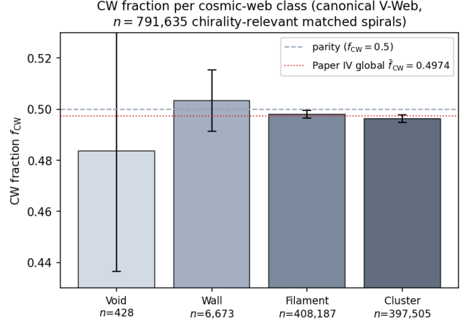
FIG. 2. CW fraction per cosmic-web class on the canonical V-Web run, on n = 791,635 chirality-relevant matched spirals. Bars show the observed f_{\text{CW}} per class; black error bars are 95% Jeffreys binomial credible intervals. The void bin ( n = 428 ) is dominated by counting noise and brackets parity. The dashed horizontal line is parity ( f_{\text{CW}} = 0.5 ); the dotted red line is the Paper IV global \bar{f}_{\text{CW}} = 0.4974 classifier-monopole offset. All four classes bracket the Paper IV monopole, consistent with no environmental dependence beyond the catalog-wide classifier bias.
