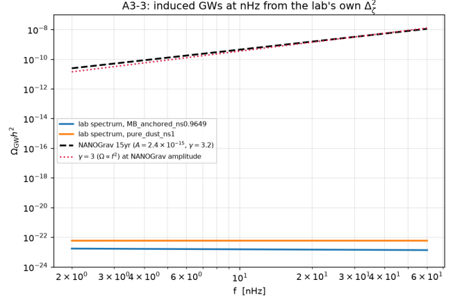
FIG. 1. Channel I null: \Omega_{\text{GW}} h^2(f) induced by this lab's own committed curvature spectrum (CMB-anchored n_s = 0.9649 and the n_s = 1 dust bracket), propagated through the validated Kohri–Terada radiation-era kernel [10] and the scale-independent A2 transfer, against NANOGrav's 15-yr power-law posterior ( \gamma_{\text{HD}} = 3.2 \pm 0.6 ). The predicted slope, \gamma_{\text{pred}} = 5.07 ( 5.00 , dust), is 5.1\sigma ( 4.9\sigma ) from the measured slope; the predicted amplitude is 10^{14.3} below the NANOGrav band. Source: outputs/sigw_nh from lab.spectrum.2026-09-04.json.
