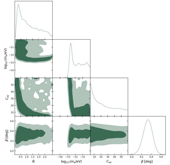
FIG. 4. Spectator-ALP joint posterior triangle from the continuous-prior cross-check configuration in which the photon anomaly coefficient is sampled freely (flat priors C_{a\gamma} \in [4, 60] — widened from the earlier [1, 30] to cover the full EOM-required band [9, 51] — \theta_i \in [0.01, \pi] , \log_{10}(m_a/\text{eV}) \in [-35, -30] — the mass prior corresponds to m/H_0 \approx 7 \times 10^{-3} to 7 \times 10^2 for H_0 = 67.7 \text{ km/s/Mpc} = 1.44 \times 10^{-33} \text{ eV} , far broader than the benchmark m/H_0 \in [1, 3] ), broadening the three fixed- C_{a\gamma} benchmark configurations of Appendix C; the direct-sample priors are on the underlying ALP parameters ( \theta_i, m_a ), with \Delta\phi/f_a derived along each trajectory. The rotation marginal, \beta = 0.326^\circ \pm 0.099^\circ , is consistent within 1\sigma with the fixed- C_{a\gamma} = 8 result \beta_{\text{ALP}} = 0.336^\circ \pm 0.107^\circ and the observed \beta_{\text{obs}} = 0.342^\circ \pm 0.094^\circ (an internal-consistency statement: all three are constrained by the same single published \beta_{\text{obs}} , not independent measurements). The \theta_i – C_{a\gamma} anti-correlation band traces the constant-product degeneracy enforced by the summary-likelihood constraint through C_{a\gamma} (\Delta\phi/f_a) \approx 10.3 , and the m_a marginal piles toward the upper (heavier) edge of its prior range — the data-driven pull toward the upper edge of the natural-prior box discussed in the text, consistent with the model accommodating rather than naturally predicting the observed rotation (fn. 5).
