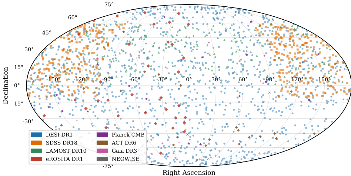
Cross-transfer baseline sky distribution: 319,443 detections across 8 archives (the released catalog uses the Path-C native re-score)
