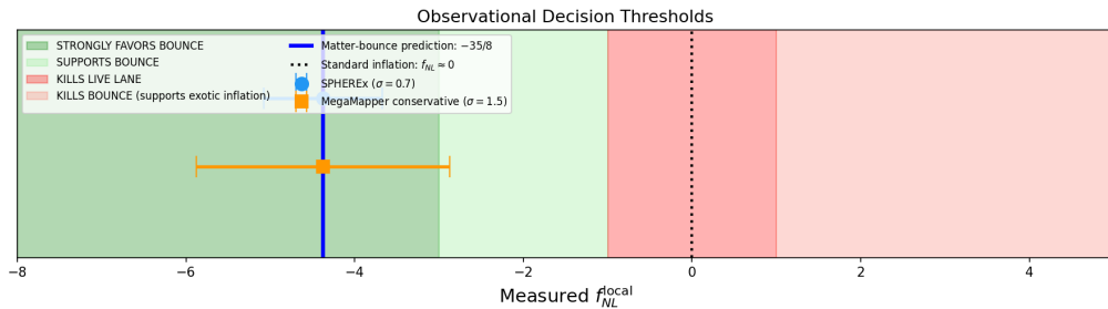
Figure 6: Observational decision thresholds. Green: strongly favors bounce. Red: strongly disfavors the quasi-dust matter bounce. Blue vertical line: bounce prediction f_{\text{NL}} = -35/8 . Error bars: SPHEREx ( \sigma = 0.7 ) and MegaMapper conservative ( \sigma = 1.5 ).
