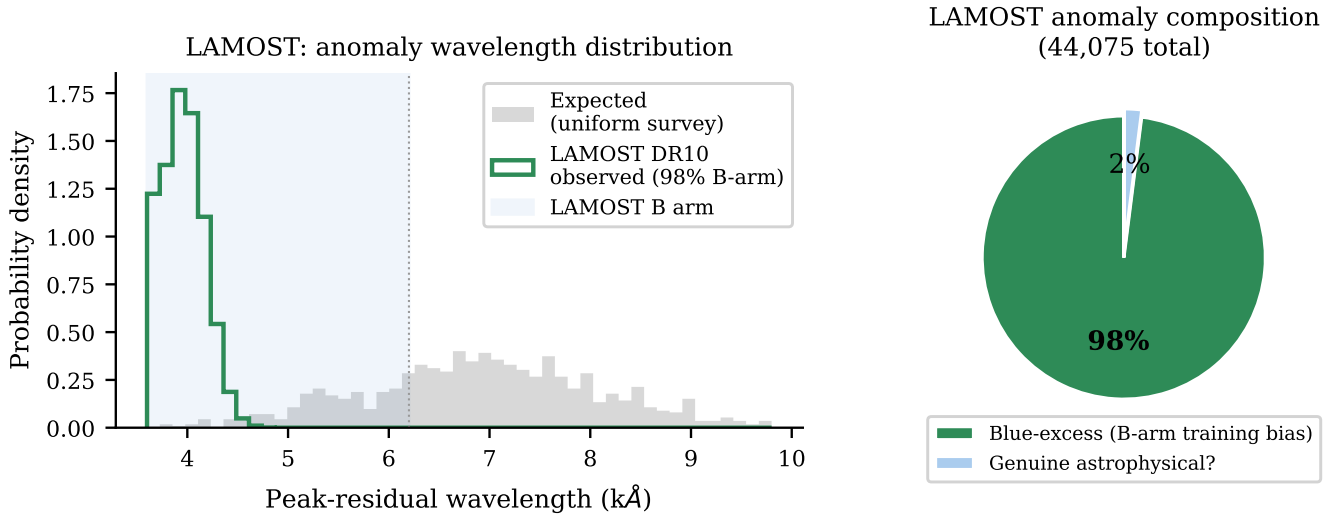
FIG. 6. LAMOST DR10 training-bias artifact. Left : Distribution of the peak-residual wavelength for LAMOST anomalies (green) vs. the expected uniform distribution (gray). The extreme concentration below 4500 Å (LAMOST B arm) — containing 98% of all anomalies — is a hallmark of training-set bias: objects observed at higher airmass or with sub-optimal blue-arm calibration are flagged as anomalous relative to a training set that does not adequately represent those conditions. Right : Composition breakdown of the 44,075 LAMOST anomalies. Only \sim 2\% pass the consistency checks expected of genuine astrophysical anomalies. This is the clearest demonstration in the paper of how an imperfect training set produces a contaminated anomaly catalog.
