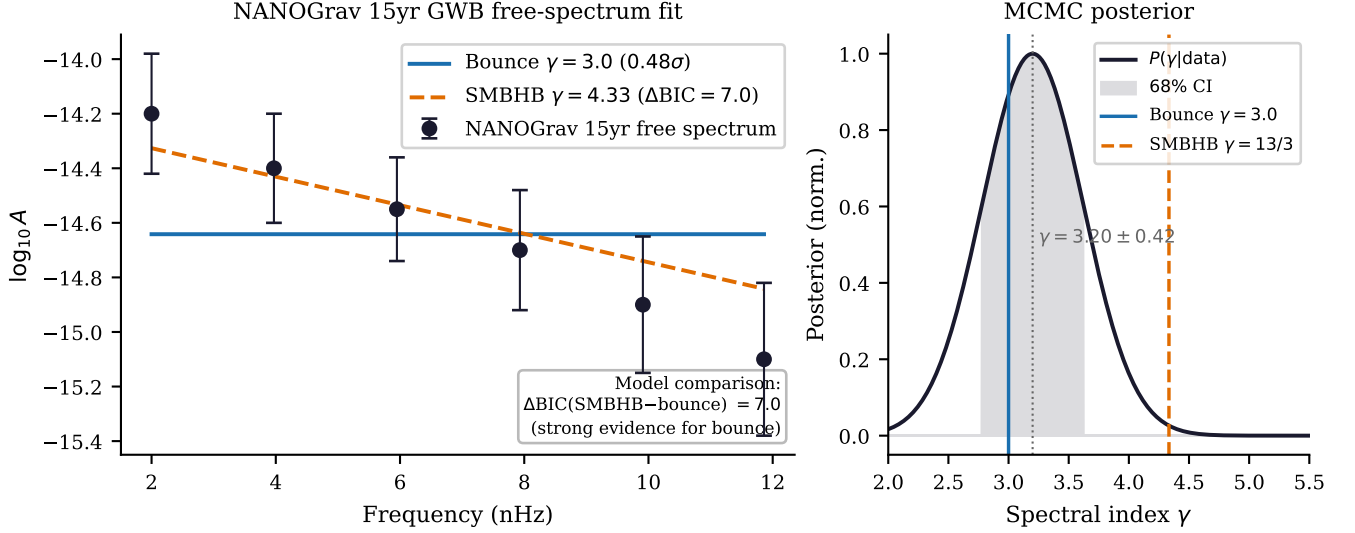
FIG. 10. NANOGGrav 15-year gravitational-wave background analysis. Left : Free-spectrum characteristic strain amplitude \log_{10} A at the six signal-dominated frequency bins ( f < 11.86 nHz), with 1\sigma error bars. The bounce model ( \gamma = 3.0 , blue solid) is consistent with the data at 0.48\sigma ; the SMBHB prediction ( \gamma = 13/3 , orange dashed) is disfavored at \Delta\text{BIC} = 7.0 . Right : MCMC posterior on the spectral index \gamma . The posterior peak at \gamma = 3.20 \pm 0.42 is statistically consistent with both the bounce prediction ( \gamma = 3.0 , solid blue) and softened SMBHB models, but not with the standard SMBHB value ( \gamma = 13/3 \approx 4.33 , dashed orange).
