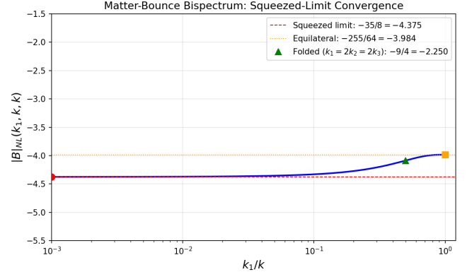
FIG. 1. Matter-bounce bispectrum shape function |B|_{\text{NL}}(k_1, k, k) as a function of the squeeze ratio k_1/k , showing convergence to -35/8 in the squeezed limit. Red circle: squeezed benchmark. Orange square: equilateral. Green triangle: folded.
