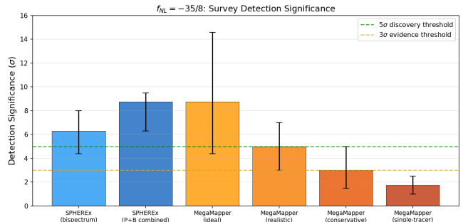
FIG. 2. Detection significance for f_{\text{NL}} = -35/8 across survey configurations. Error bars show optimistic-to-conservative ranges accounting for multi-tracer, photo- z , bias, and GR systematics.
